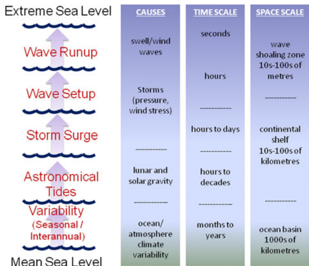
Fig. 1 Oceanic phenomena that contribute to the total water levels at the coast during an extreme sea level event, their causes and the time and space scales over which they operate
