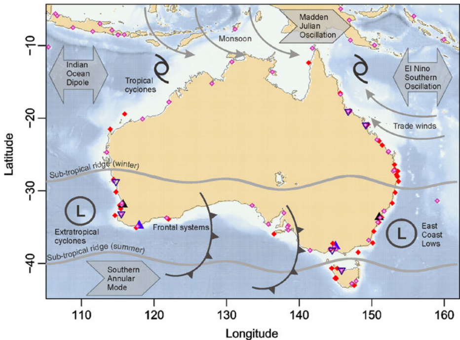
Fig. 3 Australian coastline showing tide gauge locations from the GESLA (Hunter et al. 2013) dataset (pink-filled diamonds), locations of Australia's two longest hourly digital tide gauge data (large black triangles) at Fremantle in the west commencing in 1897 and Fort Denison in the east commencing in 1914, locations where digitization could extend the hourly records to the late 19th century (large solid blue triangles) and locations where digitization could extend the hourly record back at least to 1950 (open blue triangles). Red diamonds indicate locations of wave buoy data. The weather and climate drivers discussed in relation to extreme coastal sea levels are also illustrated. Light-to-dark shading over the ocean indicates shallow-to-deep bathymetry respectively
