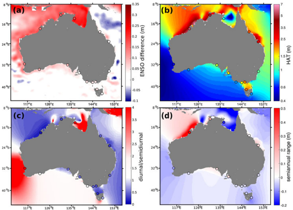
Fig. 2 Tide gauge and satellite altimetry derived ENSO-dependent sea-level differences and astronomical tidal characteristics around Australia: a differences between La Niña and El Niño sea levels conditions, defined as median monthly sea-level during periods when SOI > 1 minus periods when SOI < -1. b Highest astronomical tide (HAT) relative to MSL on a logarithmic scale. c Tide type, defined as the ratio of the amplitude of the principle diurnal constituents (K1, O1) to the semidiurnal constituents (M2, S2); when this ratio is >3 tides are considered fully diurnal in nature, <3 to >0.25 they are mixed and <0.25 they are diurnal. d Range in semiannual tidal amplitude (indicated by 2 K2 – 201 constituents); positive (negative) values indicate peak astronomical spring tides occur near the equinoxes (solstices). Black circles indicate tide gauges in the Australian Baseline Sea Level Monitoring Project network; circle interior colours indicate values derived from hourly sea-level observations; gridded data values are independently calculated from the following sources: (a) AVISO DT MSLA “all sat merged” ( www.aviso.altimetry.fr ); (b-d) TPXO7-Atlas ( volkov.oce.orst.edu/tides )
